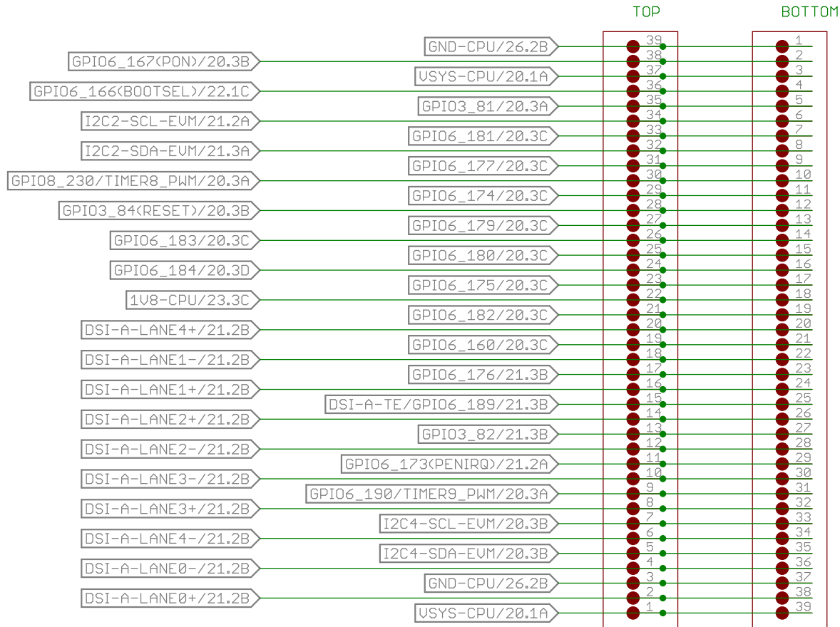
FH23-39S-0.3SHW(0.5)
