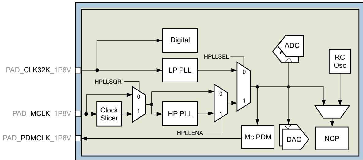
Figure 13. Clock System
